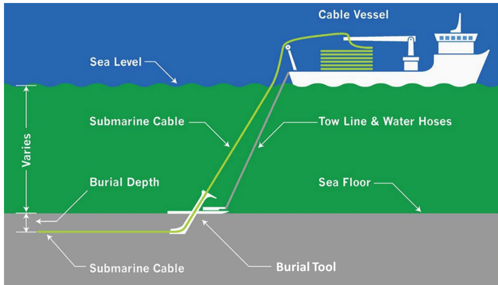
Schematic of a Cable Installation Process
